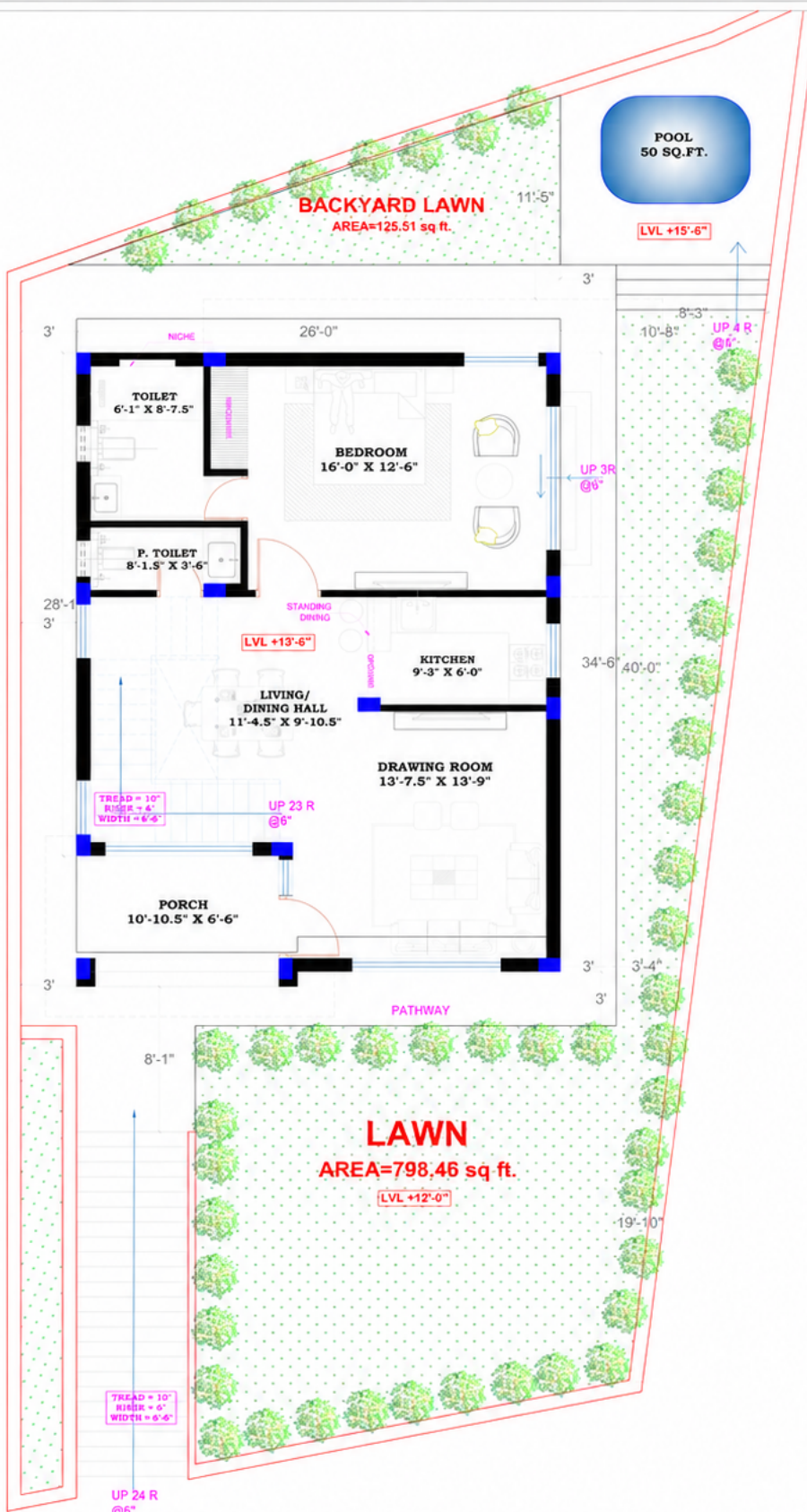
GROUND FLOOR WITH PARK & PLUNGE POOL
